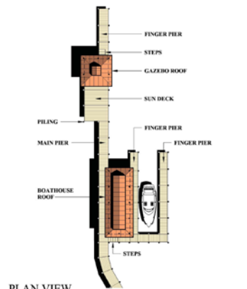
BOATHOUSE AND GAZEBO OPTIONS - SCHEME A SCALE: 1/4" = 1'-0"
