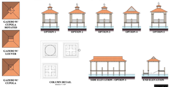
BOATHOUSE AND GAZEBO OPTIONS - SCHEME A SCALE: 1/4" = 1'-0"
